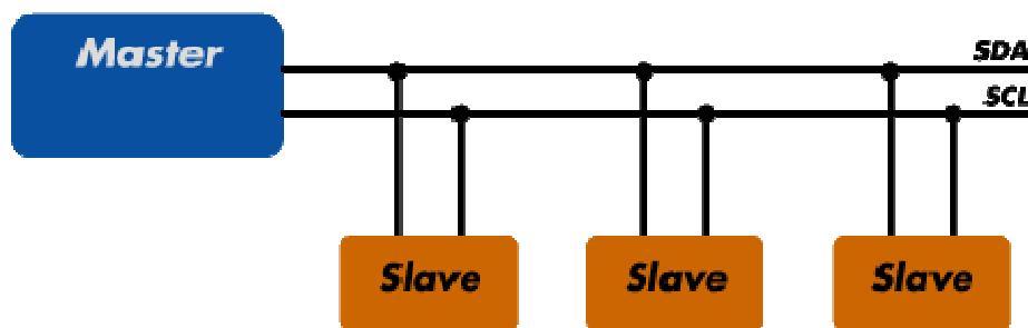
Figure 1: Sample I2C Implementation.
